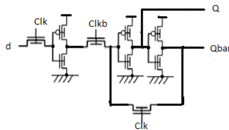
Fig 3.SG-FINFET SET D Flip flop implementation
