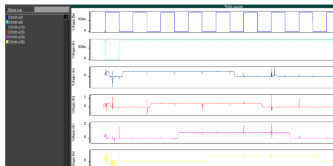
Fig 6. Johnson counter
