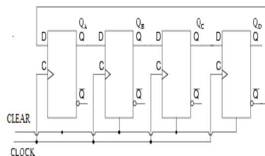
Fig 4. Johnson counter
