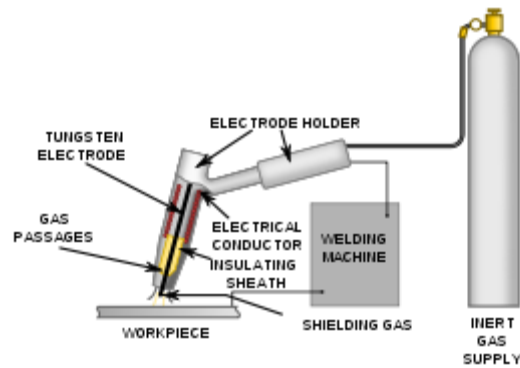
Schematic diagram of TIG welding shown in figure 1.
